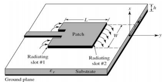
Figure 1: The Radiation of the Microstrip Patch Antenna [5].
